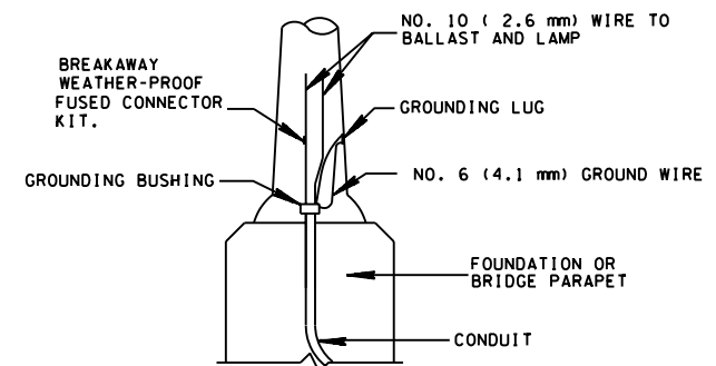
CONNECTION DETAIL
