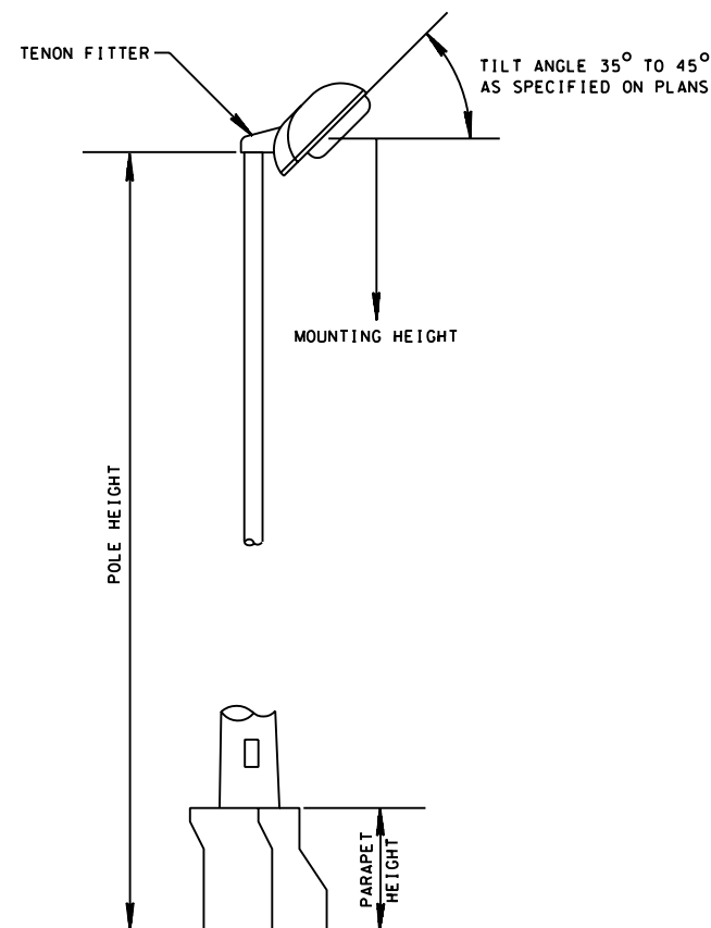
LIGHT STANDARD DETAIL BRIDGE MOUNTED
