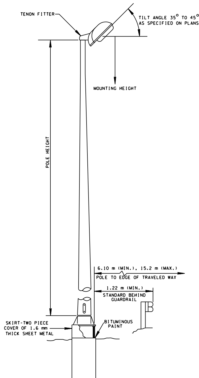
LIGHT STANDARD DETAIL GROUND MOUNTED
